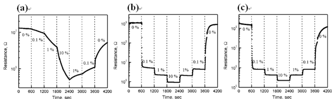
Fig. 3. Typical sensor response of (a) pure \text{TiO}_2 nanotube layer, (b) Pt additional \text{TiO}_2 nanotube layer, and (c) Pd additional \text{TiO}_2 nanotube layer at 290^\circ\text{C} to different concentrations of hydrogen in the 0~10 vol% range.
