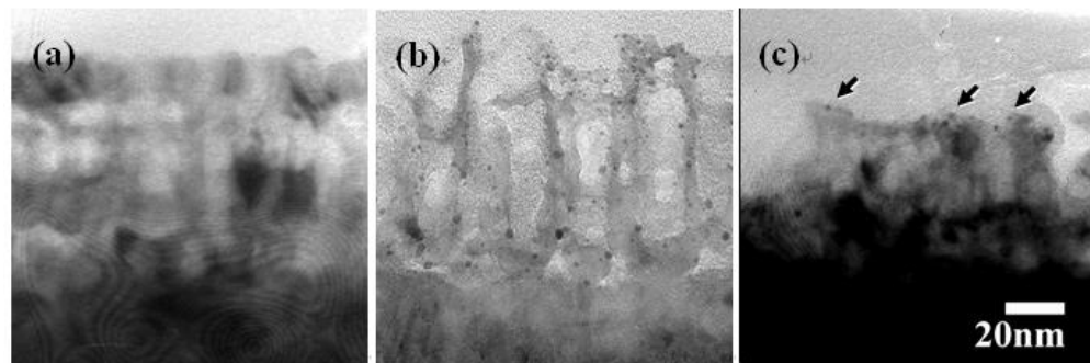
Fig. 5. FE-TEM cross-sectional micro-topography of the tubular part of \text{TiO}_2 nanotubes formed on (a) pure Ti-IBSD thin film, (b) Pt-added Ti-IBSD thin film, and (c) Pd-added Ti-IBSD thin film in glycerol and water mixture (Vol 1:1) added with 0.5wt% \text{NH}_4\text{F} .
