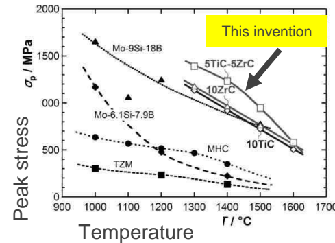
Temperature dependency of peak stress after homogenization heat treatment on high temperature compression test of this invention Mo-Si-B alloy
