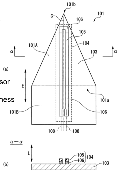
【Up left】Squint view of this invention 【Up right】Ground plan and cross section of cantilever equipped with this invention 【Down left】Impedance results (absolute value) against the magnetostriction layer's bending value of this vibration sensor
